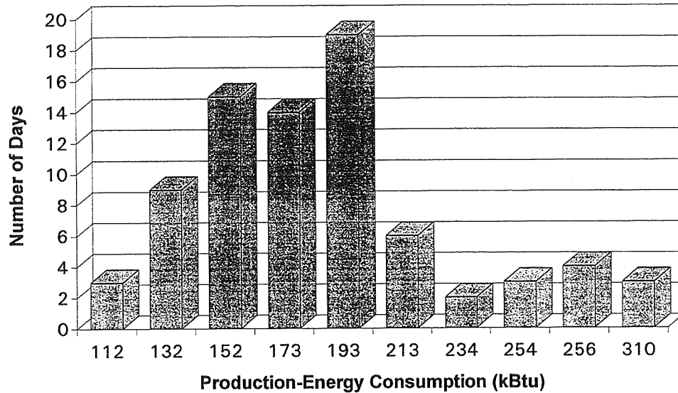
Figure C-1. Frequency of cooktop daily production energy consumption.
