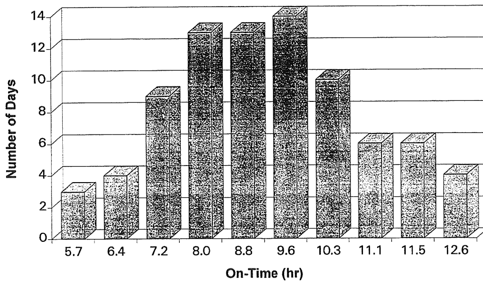
Figure C-2. Frequency of cooktop daily on-time.
