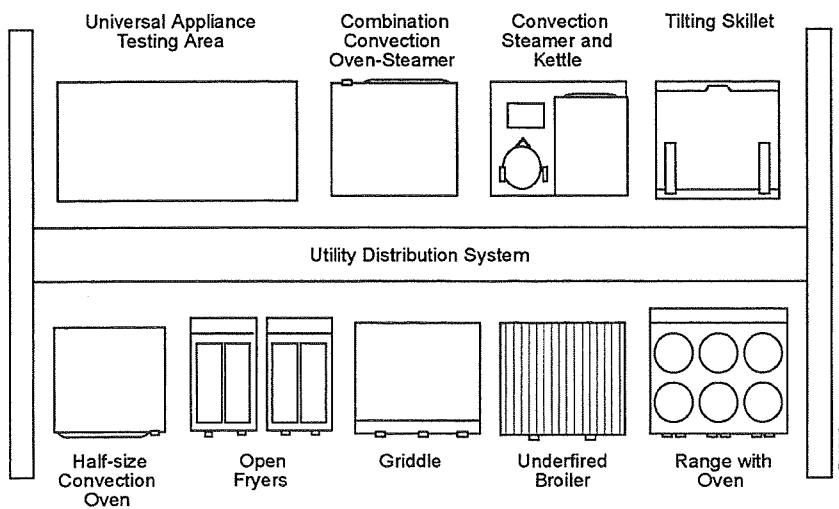
Figure 1-2. The production center.
