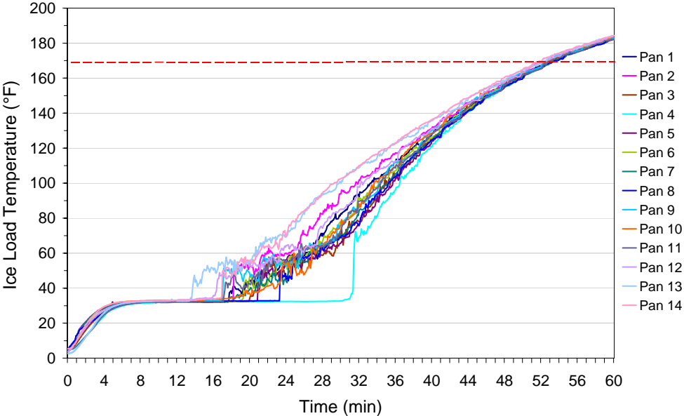
Figure 3-4. Ice-load temperature profile.
