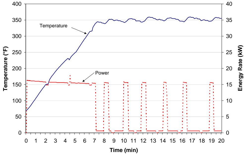
Preheat Curve
