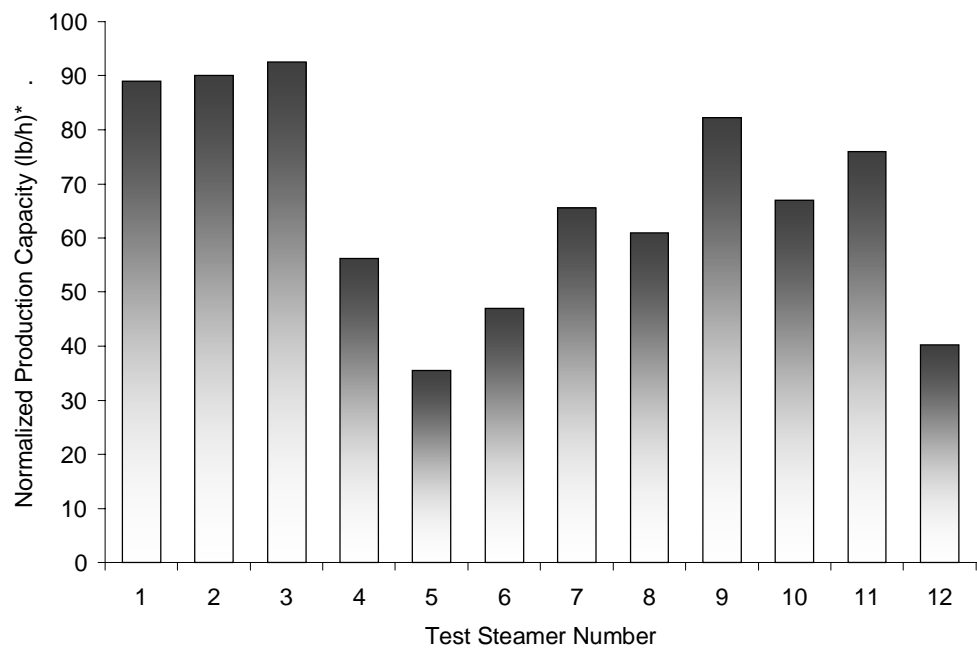
Figure 8-7. Normalized electric pressureless steamer production capacity.
