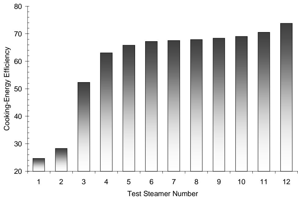
Figure 8-8. Electric pressureless steamer cooking-energy efficiency.
