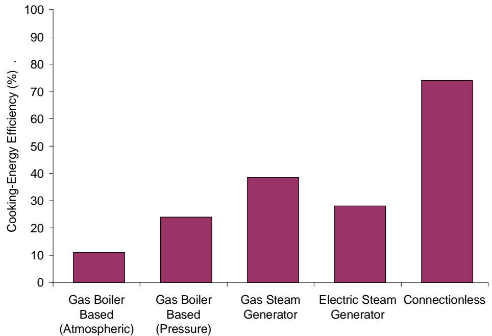
Figure 8-6. Typical red potato cooking-energy efficiencies of steamers.
