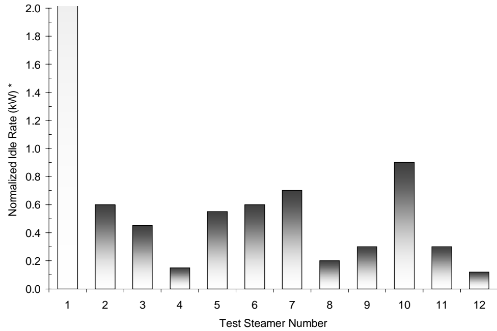
Figure 8-4. Normalized electric pressureless steamer idle energy rates.
