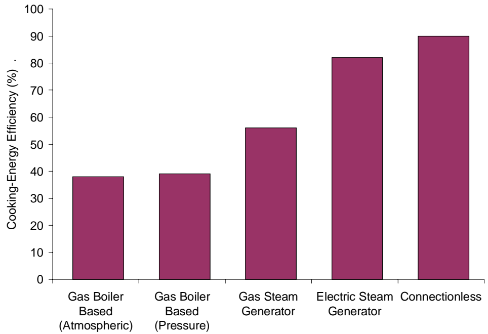
Figure 8-5. Typical frozen green pea cooking-energy efficiencies of steamers.
